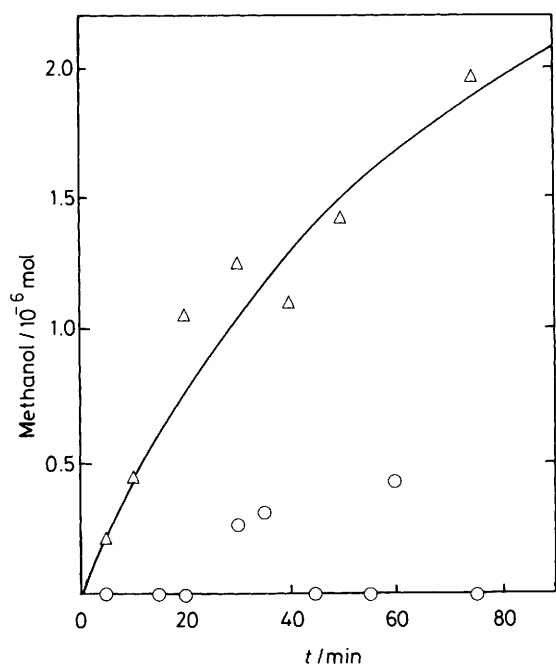
Figure 1 Time dependence of methanol formation. The sample solution (total volume 3.0 ml) contains cell suspension (0.5 ml), methane ( 1.0 \times 10^{-4} mol), oxygen ( 8.0 \times 10^{-5} mol), and \text{HCO}_2\text{Na} ( 5.0 \times 10^{-5} mol) in phosphate buffer ( 3.0 \times 10^{-2} M) (pH 7.0). The reaction was carried out at 30°C. \Delta : cyclopropane treated cells, \circ : non-treated cells.
